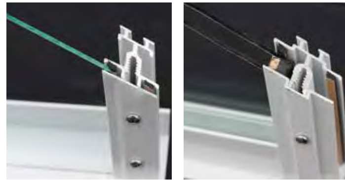
SINGLE PANE GLAZING
